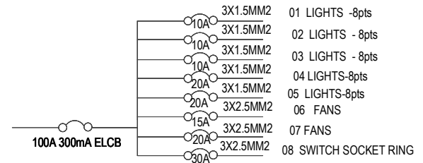
8WAYS TPN DISTRIBUTION BOARD SURGICAL AND MEDICAL WARD
