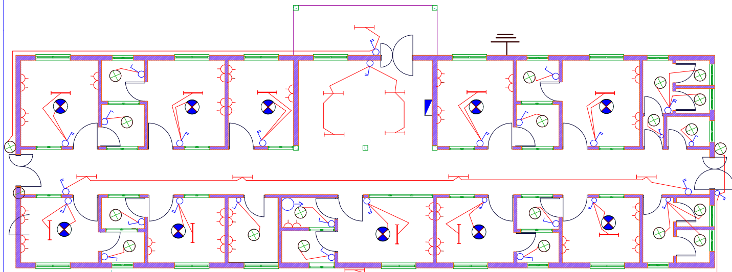
8WAYS TPN DISTRIBUTION BOARD GRADE 1 WARD
