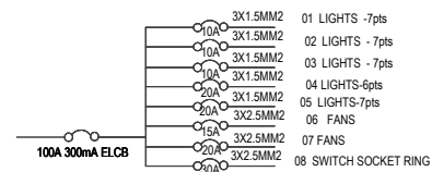
8WAYS TPN DISTRIBUTION BOARD 2 ADM
