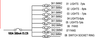
8WAYS TPN DISTRIBUTION BOARD 1 ADM
